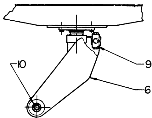
VIEW B-B
