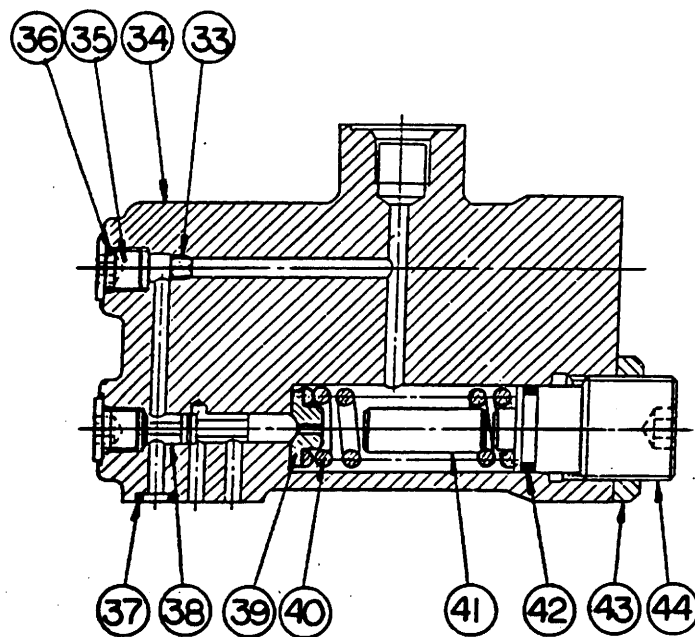
COMPENSATOR ASS'Y.
